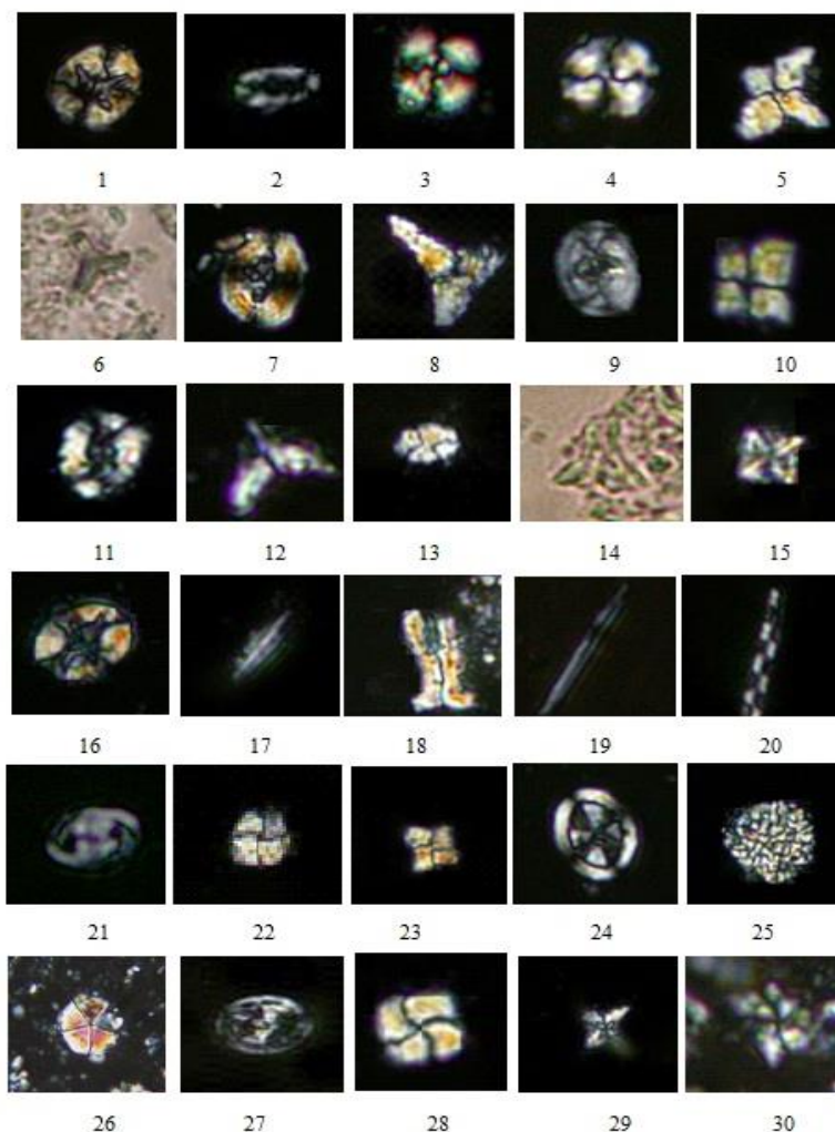
Plate: All figures magnification of \times 1000 . 1. Eiffelithus turriseiffelii (Deflandre in Deflandre & Fert, 1954) Reinhardt, 1965, (XPL); 2. Rhagodiscus angustus (Stradner, 1963) Reinhardt, 1971, (XPL); 3. Watznaueria 4. Watznaueria biporta Bukry, barnesiae (Black in Black & Barnes, 1959) Perch-Nielsen, 1968, (XPL); 1969; (XPL); 5. Quadrum sissinghii Perch-Nielsen (1984b), (XPL); 6. Marhasterites furcatus (Deflandre in Deflander and Fert, 1954) Deflander, 1959, (PPL); 7. Aspidolithus parvus constrictus (Hattner et al., 1980) Perch-Nielsen (1984a), (XPL); 8. Quadrum trifidum (Stradner) Prins & Perch-Nielsen 1977, (XPL); 9. Reinhardtites levis Prins & Sissingh in Sissingh, 1977, (XPL); 10. Quadrum gothicum (Deflandre, 1959) Prins & Perch-Nielsen in Manivit et al. (1977); 11. Aspidolithus parvus parvus (Stradner, 1963) Noel (1969); 12. Ceratolithoides arcuatus Prins & Sissingh in Sissingh, 1977, (XPL); 13. Calculites obscurus (Deflandre, 1959) Prins & Sissingh in Sissingh (1977), (XPL); 14. Ceratolithoides verbeekii Perch-Nielsen, 1979, (XPL); 15. Micula decussata Vekshina (1959), (XPL); 16. Eiffelithus eximius (Stover, 1966) Perch-Nielsen, 1968, (XPL); 17. Lithraphidites quadratus Bramlette & Martini (1964), (XPL); 18. Lucianorhabdus cayeuxii Deflandre, 1959, (XPL); 19. Lithraphidites carniolensis Deflander, 1963, (XPL); 20. Microrhabdulus decoratus Deflandre, 1959, (XPL); 21. Tranolithus orionatus (Reinhardt, 1966a) Reinhardt, 1966b (XPL); 22. Calculites ovalis (Stradner, 1963) Prins & Sissingh in Sissingh (1977), (XPL); 23. Micula murus (Martini, 1961) Bukry (1973), (XPL); 24. Arkhangelskiella cymbiformis Vekshina, 1959, (XPL); 25. Thoracosphaera operculata Bramlette & Martini (1964), (XPL); 26. Braarudosphaera bigelowii (Gran & Braarud 1935) Deflandre 1947, (XPL); 27. Reinhardtites anthophorus (Deflandre, 1959) Perch-Nielsen (1968), (XPL); 28. Micula praemurus (Bukry, 1973) Stradner & Steinmetz (1984); 29. Micula staurophora (Gardet, 1955) Stradner, 1963, (XPL); 30. Lithastrinus grillii Stradner (1962), (XPL).
